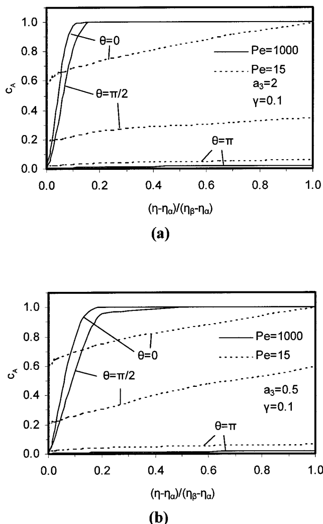
Figure 2. Concentration profiles for prolate (a) and oblate (b) spheroidal shapes for a high and a low Peclet number at three different angular positions.
