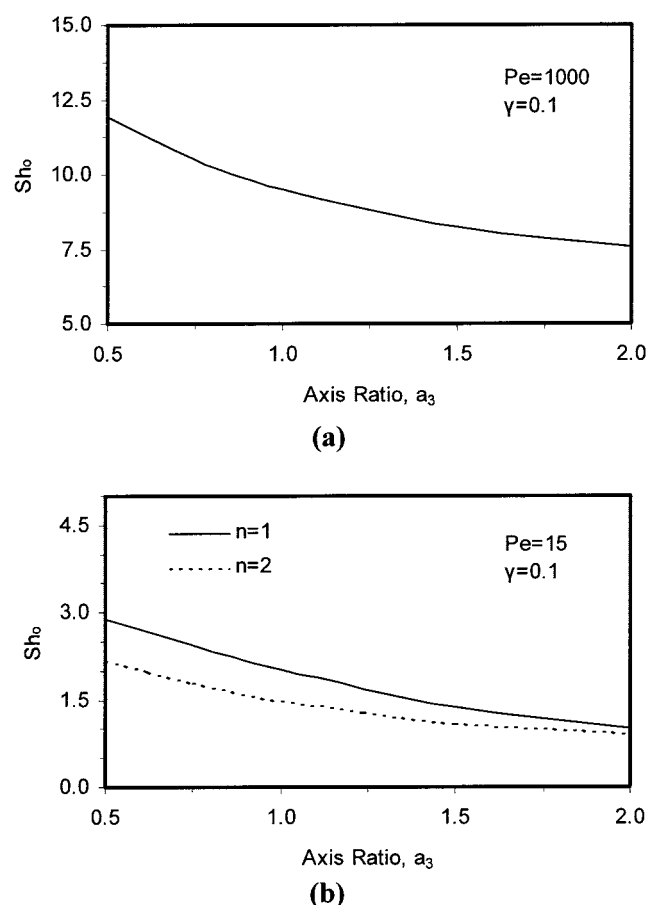
Figure 3. Dependency of the overall Sherwood number on the axis ratio of the spheroid for a high (a) and a low (b) Peclet number.
